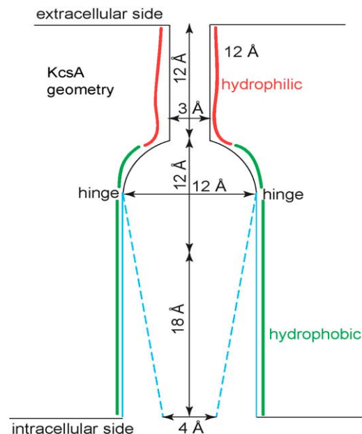
FIGURE 4 A simplified model of the KcsA channel. In our model, bubbles form on the hydrophobic side of the channel below the semi-spherical cavity. The hydrophilic selectivity filter is on the extracellular side. The hydrophobic gate is shown in two possible conformations, starting from a diameter of d_2 = 12 \text{ \AA} and closing to diameter d_2 = 4 \text{ \AA} . We consider bubble formation as d_2 changes. Confinement by a hydrophobic region is required to make bubbles persist long enough to observe them or their biological effects, i.e., to make bubbles stable.
